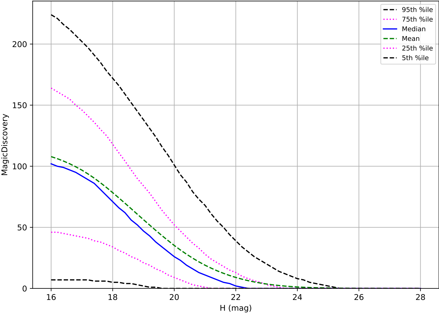
too_elab_heavy_r64_d2_griz_v3.4_10yrs: PHA 6 detections in 60 nights detection loss
