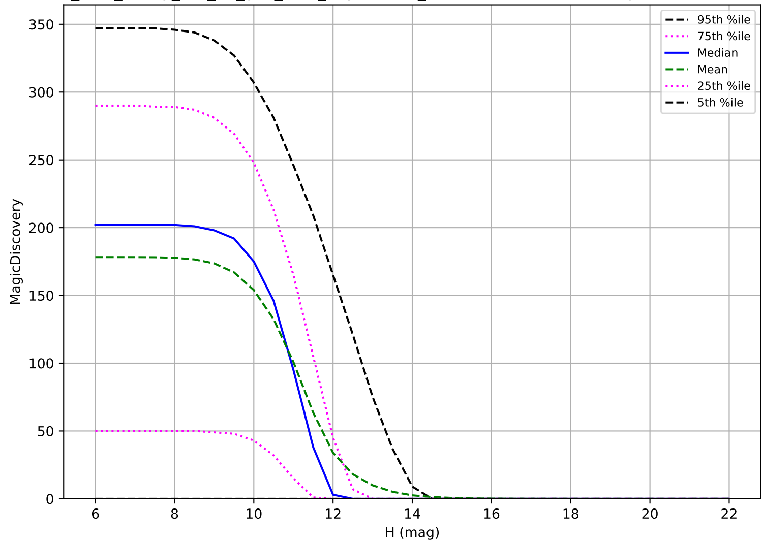
too_elab_heavy_r64_d2_griz_v3.4_10yrs: OCC_r20 6 detections in 60 nights detection loss
