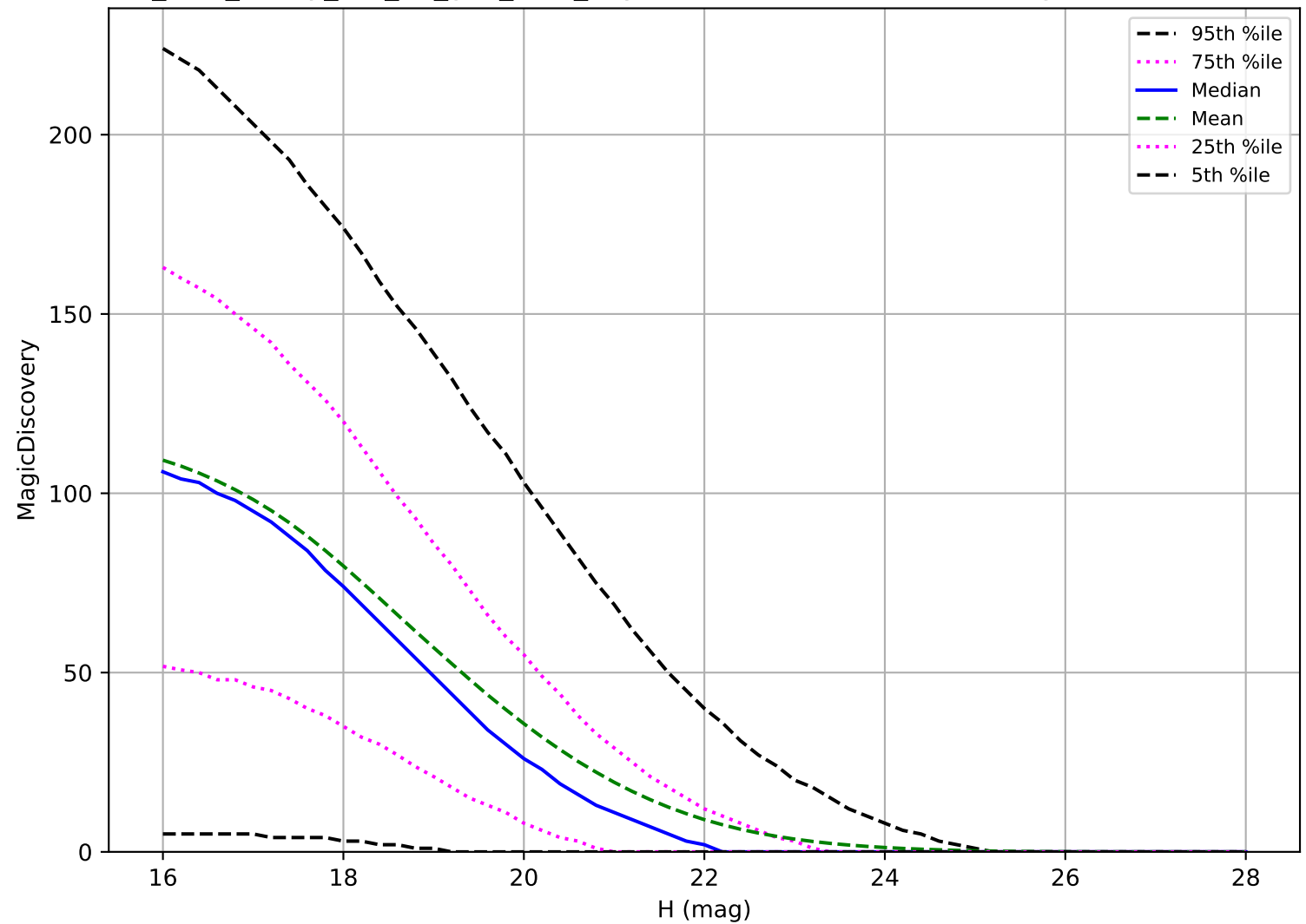
too_elab_heavy_r64_d2_griz_v3.4_10yrs: NEO 6 detections in 60 nights detection loss
