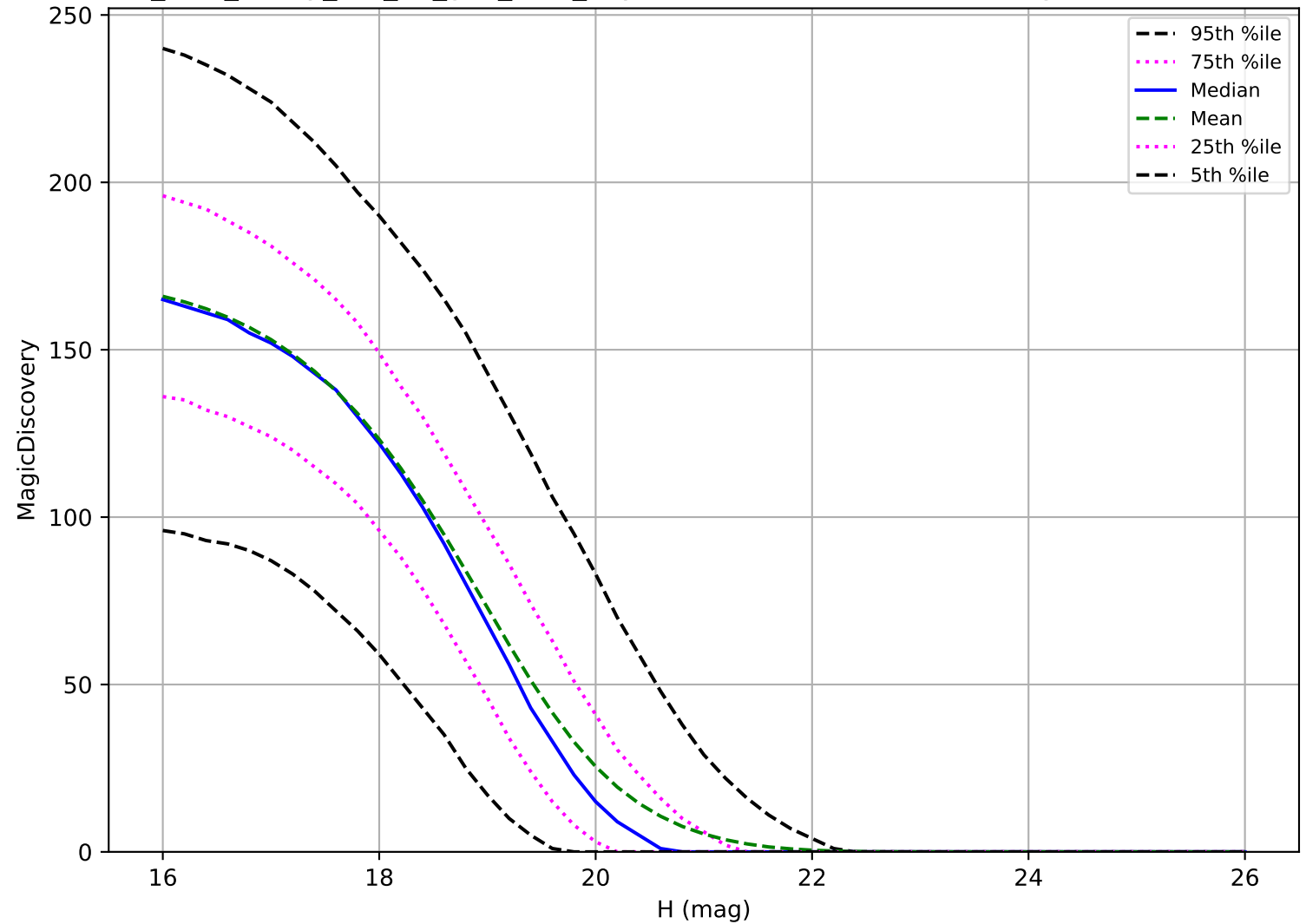
too_elab_heavy_r64_d2_griz_v3.4_10yrs: MBA 6 detections in 60 nights detection loss
