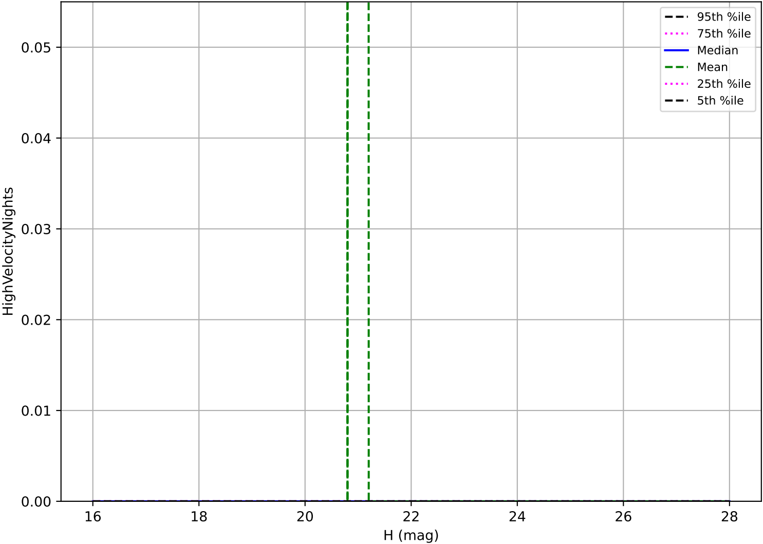
too_elab_heavy_r64_d2_griz_v3.4_10yrs: Vatira High velocity pair detection loss
