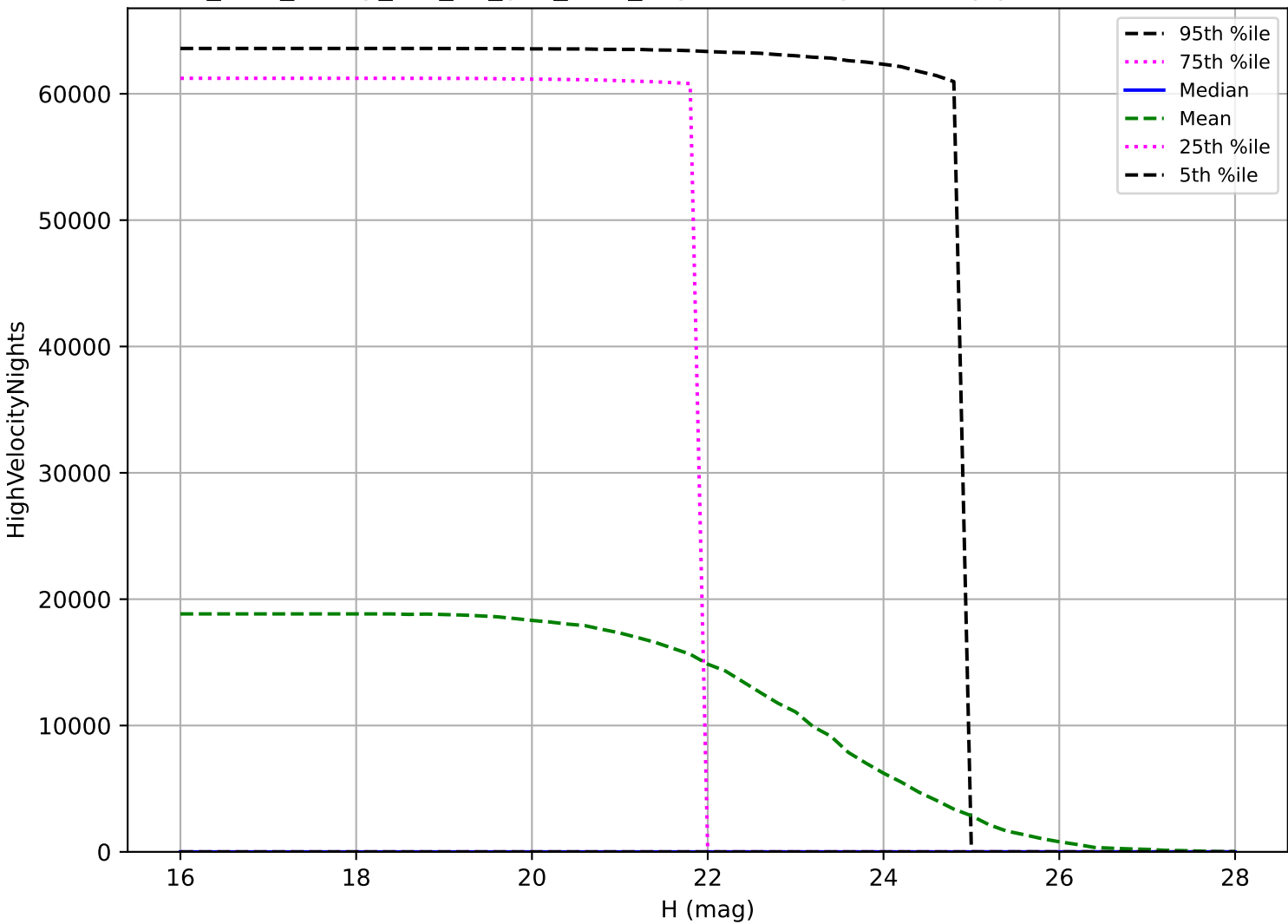
too_elab_heavy_r64_d2_griz_v3.4_10yrs: NEO High velocity pair detection loss
