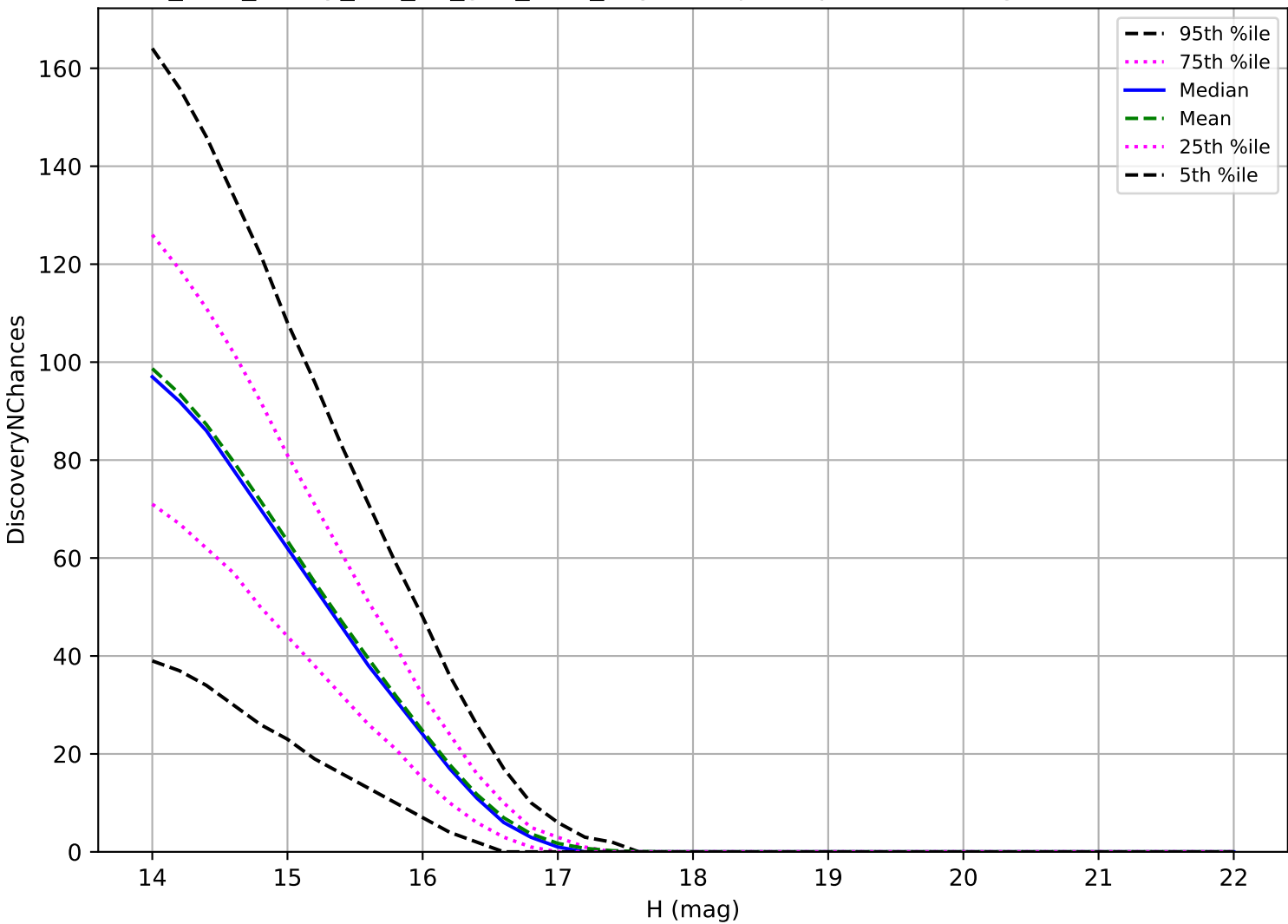
too_elab_heavy_r64_d2_griz_v3.4_10yrs: Trojan 3 pairs in 15 nights detection loss
