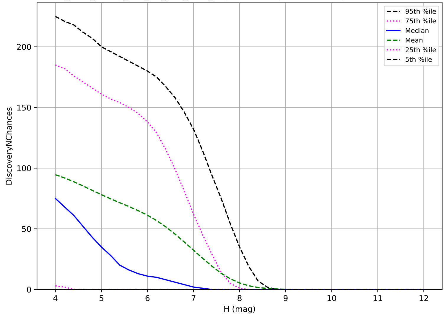
too_elab_heavy_r64_d2_griz_v3.4_10yrs: TNO 3 pairs in 15 nights detection loss
