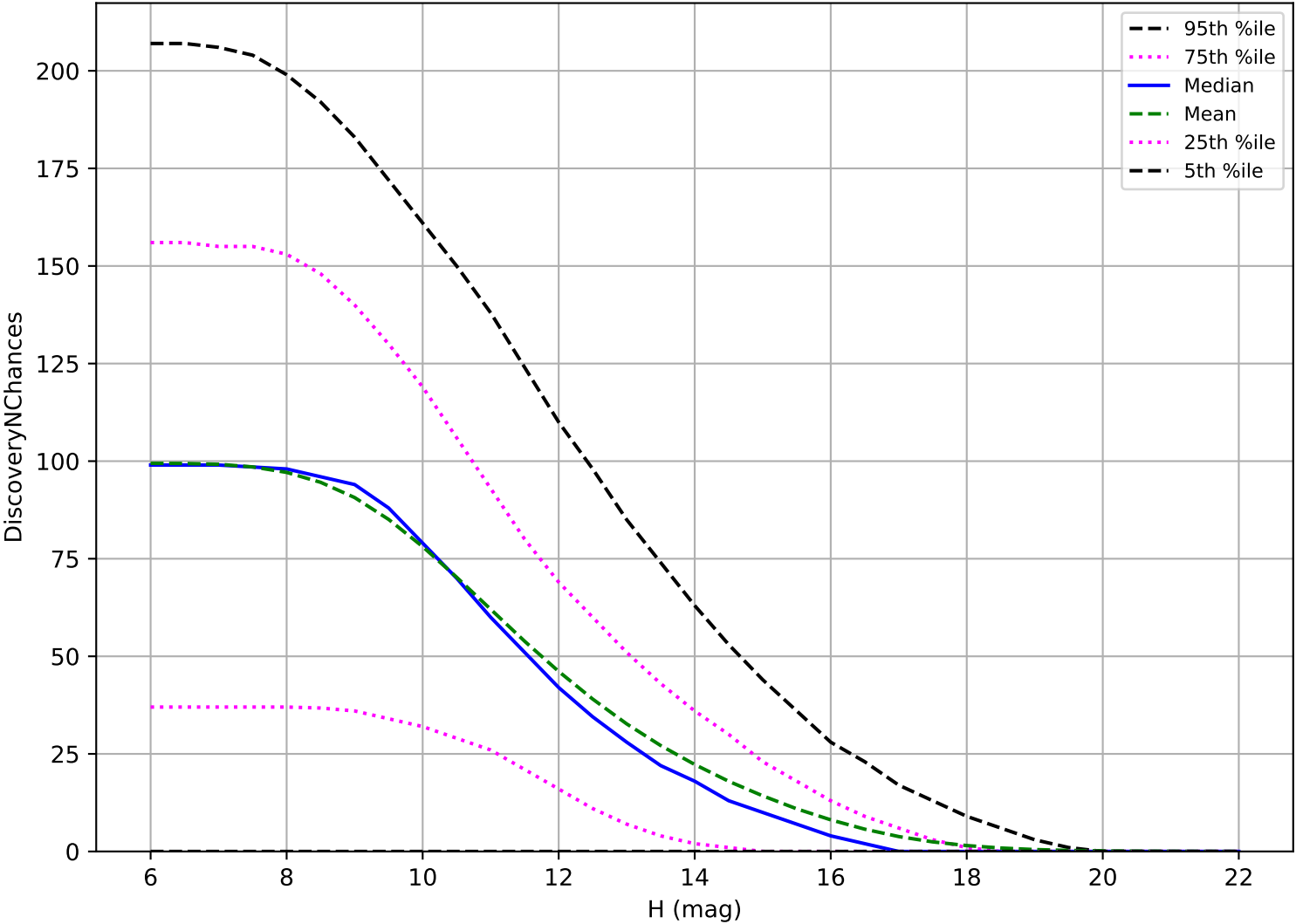
too_elab_heavy_r64_d2_griz_v3.4_10yrs: OCC_r5 3 pairs in 15 nights detection loss
