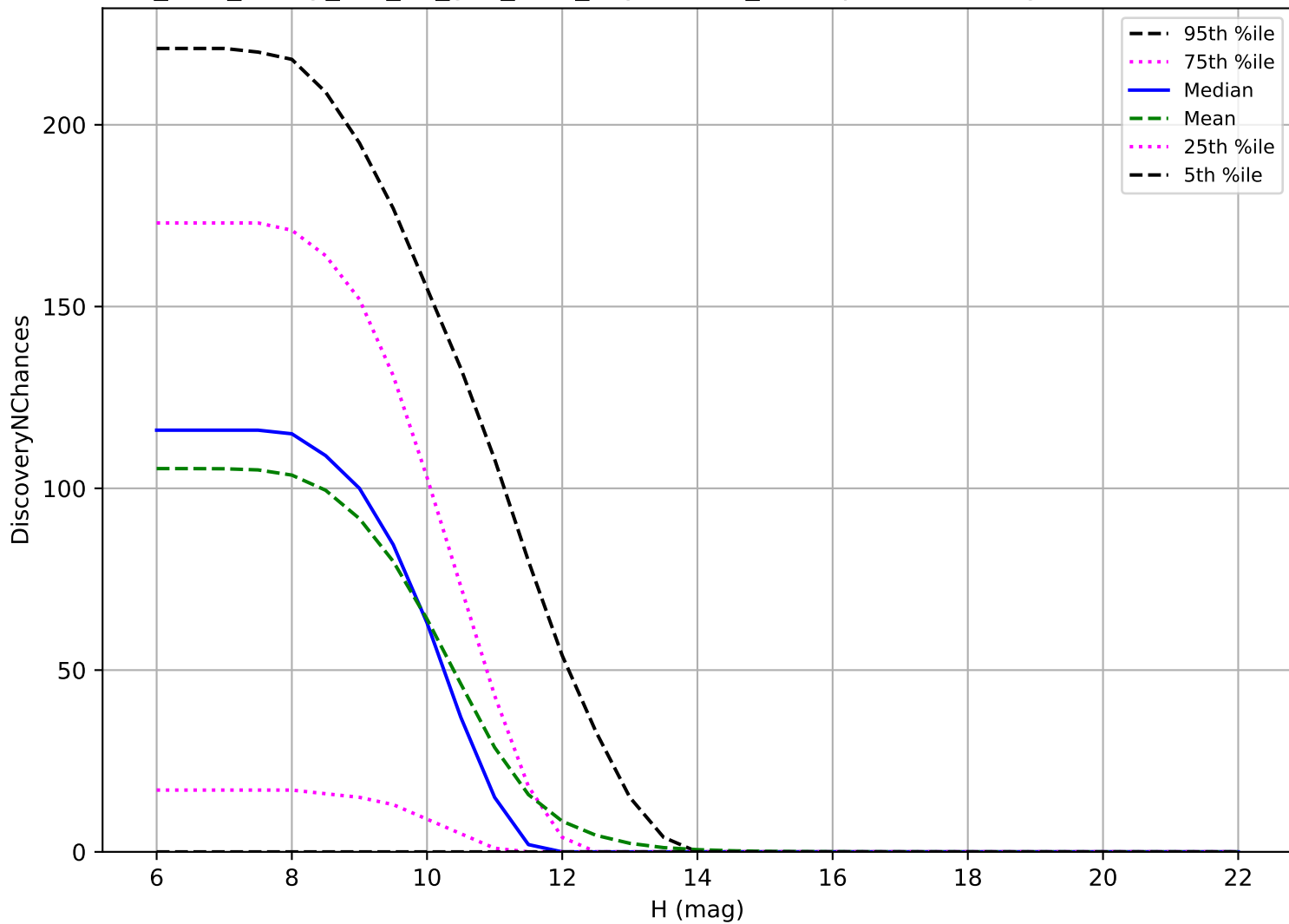
too_elab_heavy_r64_d2_griz_v3.4_10yrs: OCC_r20 3 pairs in 15 nights detection loss
