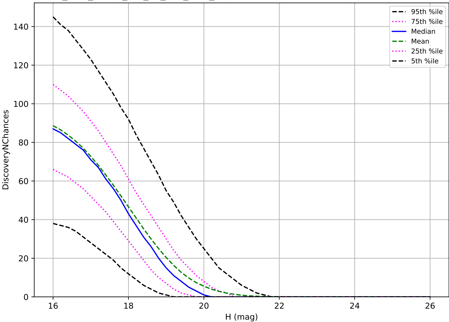
too_elab_heavy_r64_d2_griz_v3.4_10yrs: MBA 3 pairs in 15 nights detection loss
