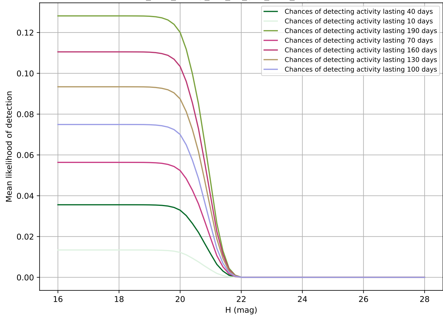
too_elab_heavy_r64_d2_griz_v3.4_10yrs Vatira
