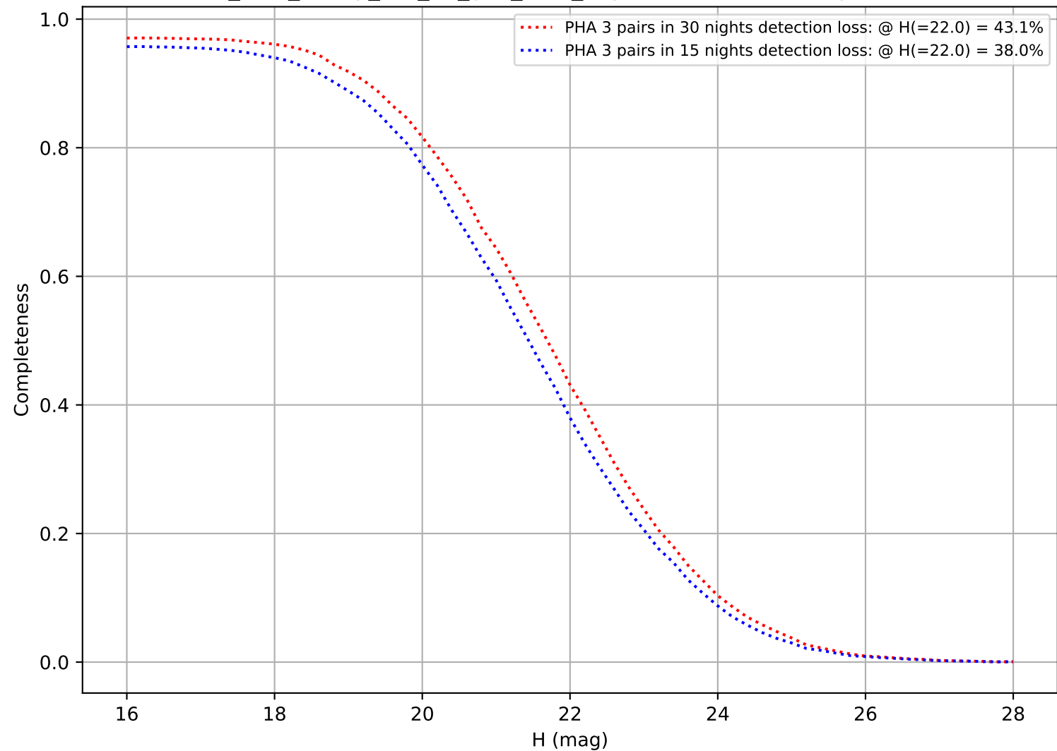
too_elab_heavy_r64_d2_griz_v3.4_10yrs: DifferentialCompleteness
