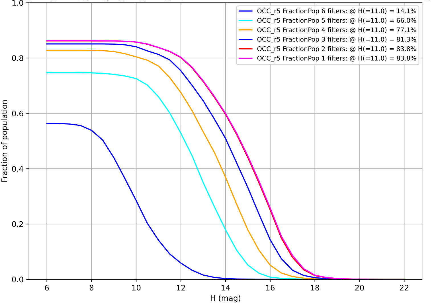
too_elab_heavy_r64_d2_griz_v3.4_10yrs: Fraction of population with colors in X filters OCC_r5
