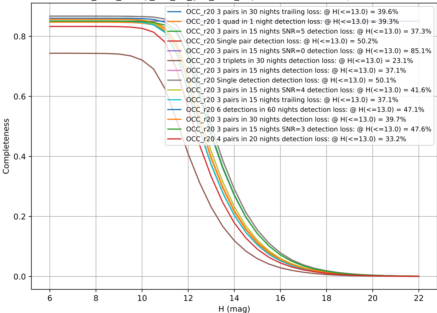
too_elab_heavy_r64_d2_griz_v3.4_10yrs: CumulativeCompleteness
