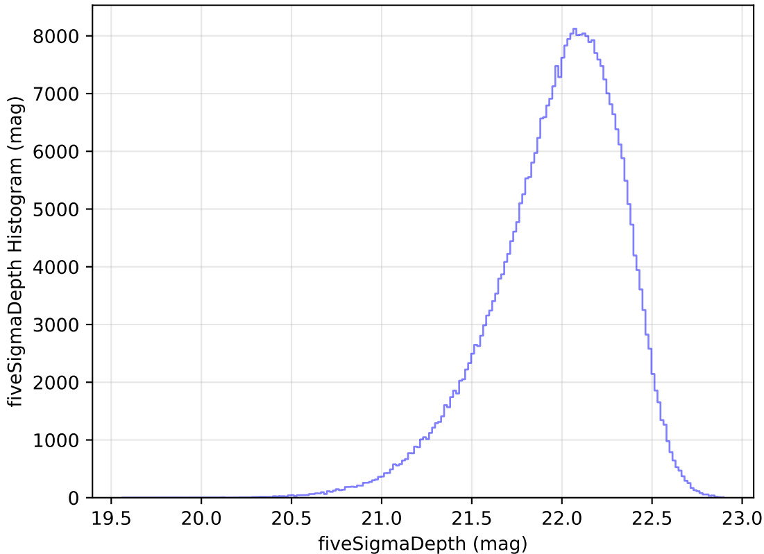
too_elab_heavy_r64_d2_griz_v3.4_10yrs y: fiveSigmaDepth Histogram
