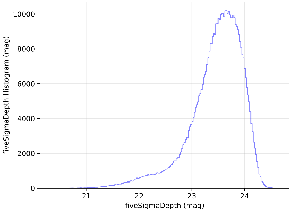
too_elab_heavy_r64_d2_griz_v3.4_10yrs i: fiveSigmaDepth Histogram
