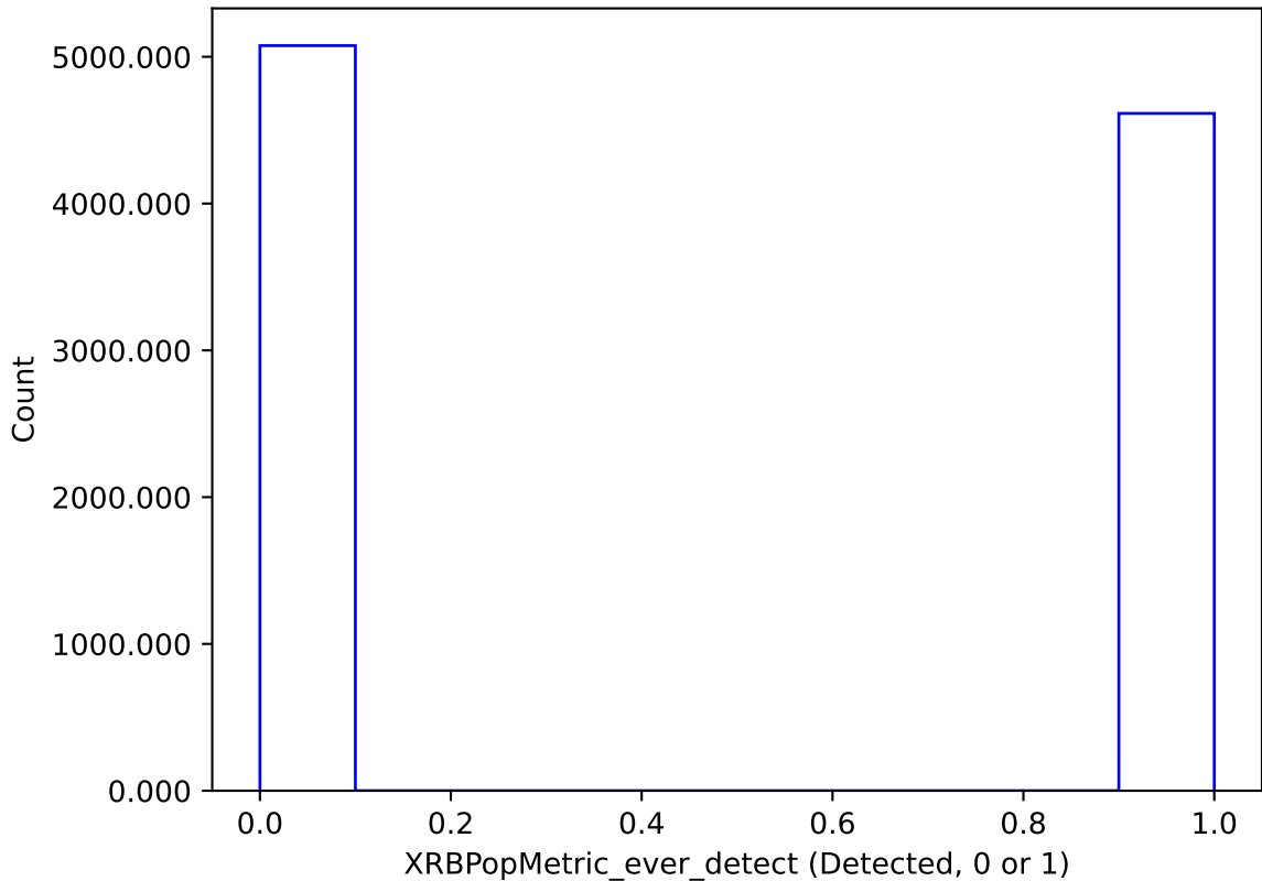
too_elab_heavy_r64_d2_griz_v3.4_10yrs : XRBPopMetric_ever_detect
