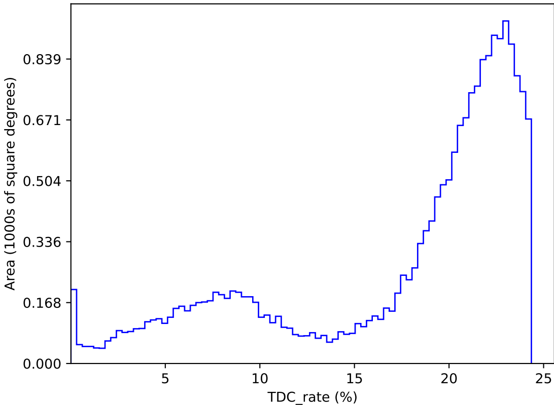
too_elab_heavy_r64_d2_griz_v3.4_10yrs : TDC_rate
