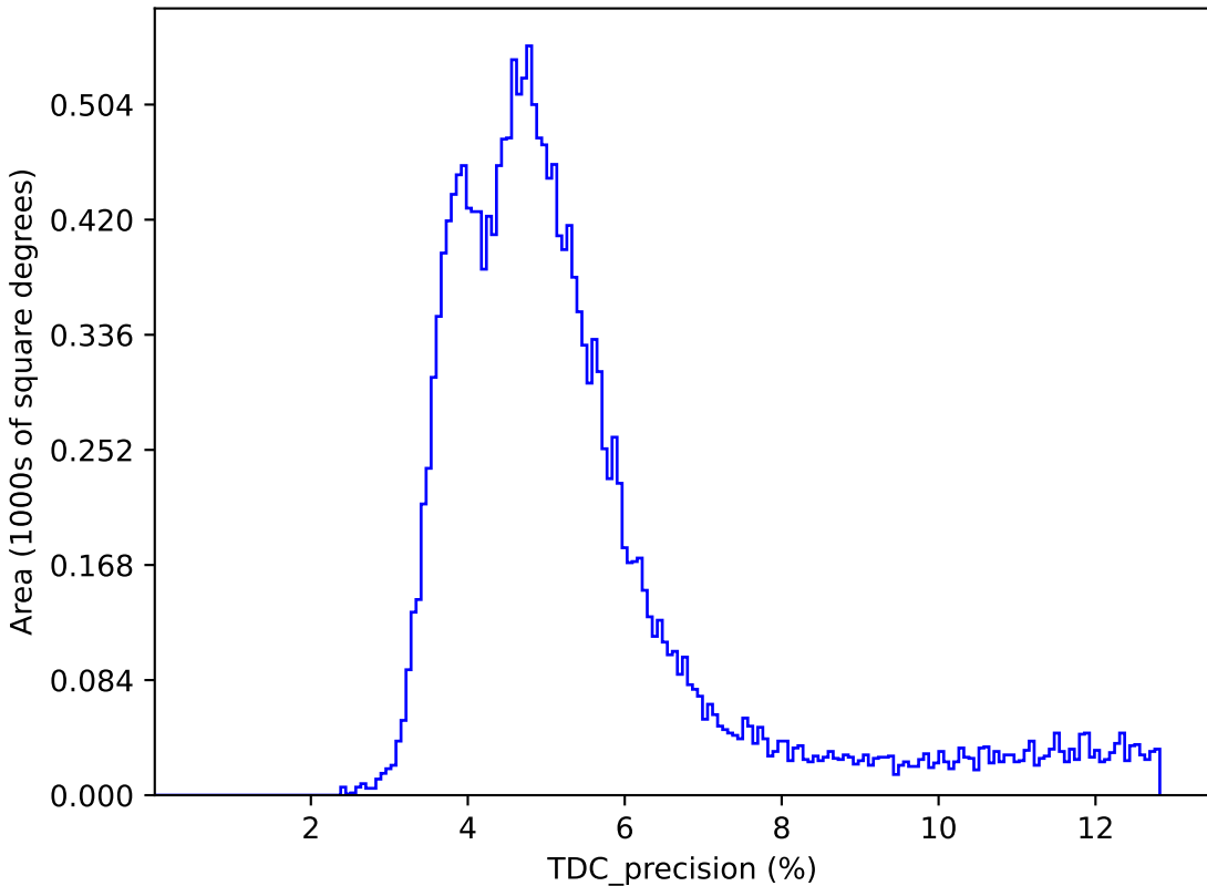
too_elab_heavy_r64_d2_griz_v3.4_10yrs : TDC_precision
