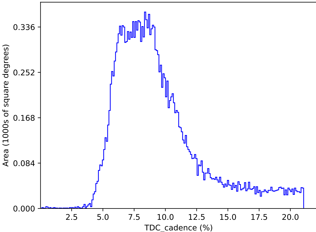
too_elab_heavy_r64_d2_griz_v3.4_10yrs : TDC_cadence
