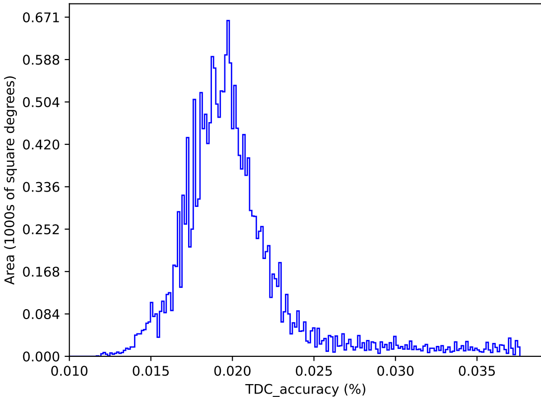
too_elab_heavy_r64_d2_griz_v3.4_10yrs : TDC_accuracy
