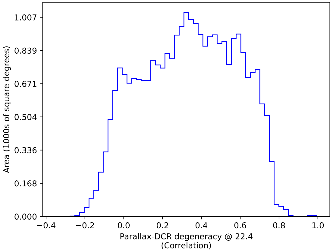
too_elab_heavy_r64_d2_griz_v3.4_10yrs : Parallax-DCR degeneracy @ 22.4
