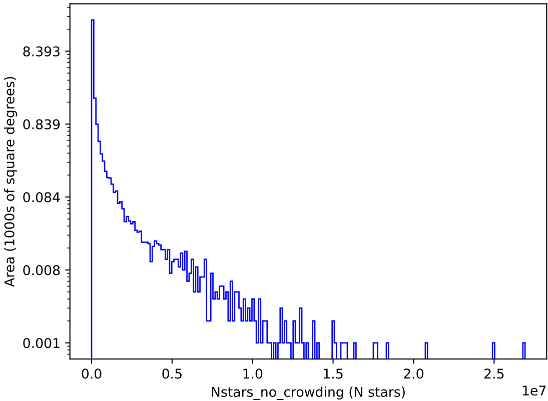
too_elab_heavy_r64_d2_griz_v3.4_10yrs z: Nstars_no_crowding
