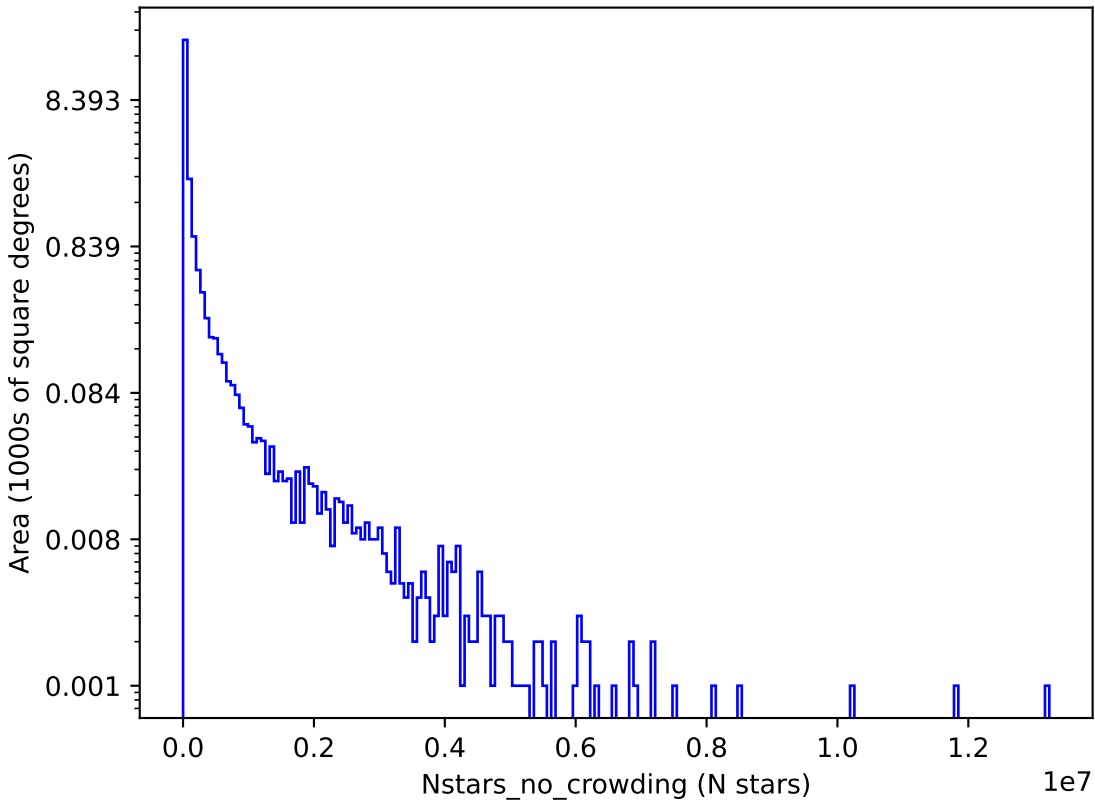
too_elab_heavy_r64_d2_griz_v3.4_10yrs g: Nstars_no_crowding
