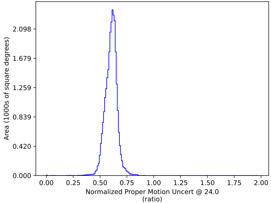
too_elab_heavy_r64_d2_griz_v3.4_10yrs : Normalized Proper Motion Uncert @ 24.0
