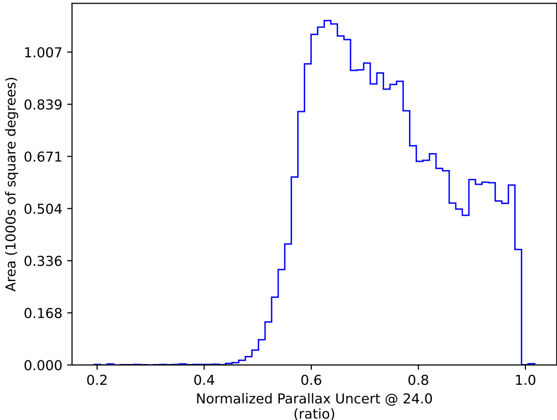
too_elab_heavy_r64_d2_griz_v3.4_10yrs : Normalized Parallax Uncert @ 24.0
