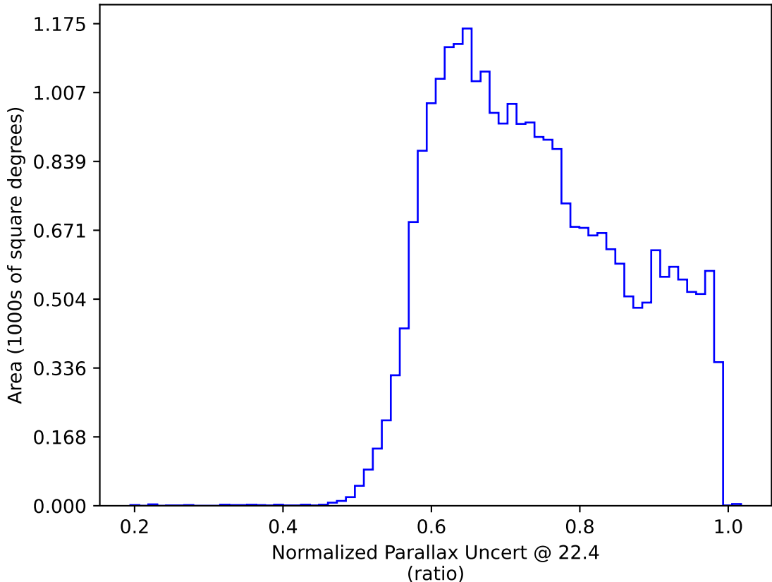
too_elab_heavy_r64_d2_griz_v3.4_10yrs : Normalized Parallax Uncert @ 22.4
