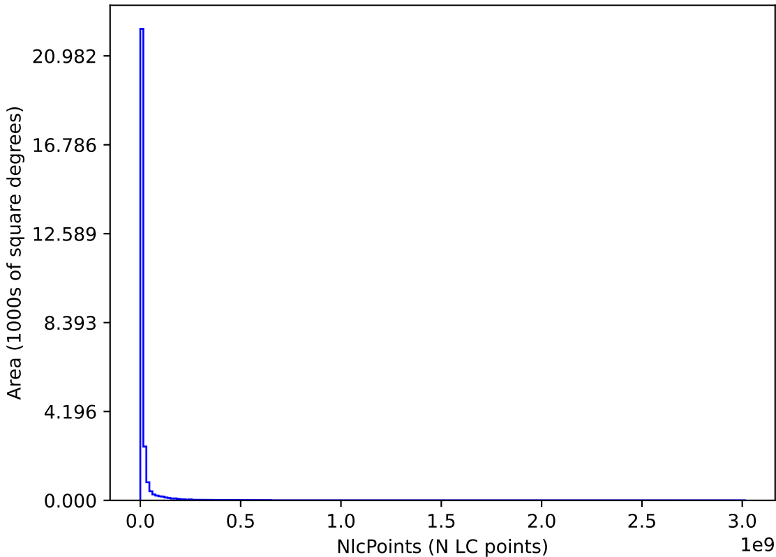
too_elab_heavy_r64_d2_griz_v3.4_10yrs : NlcPoints
