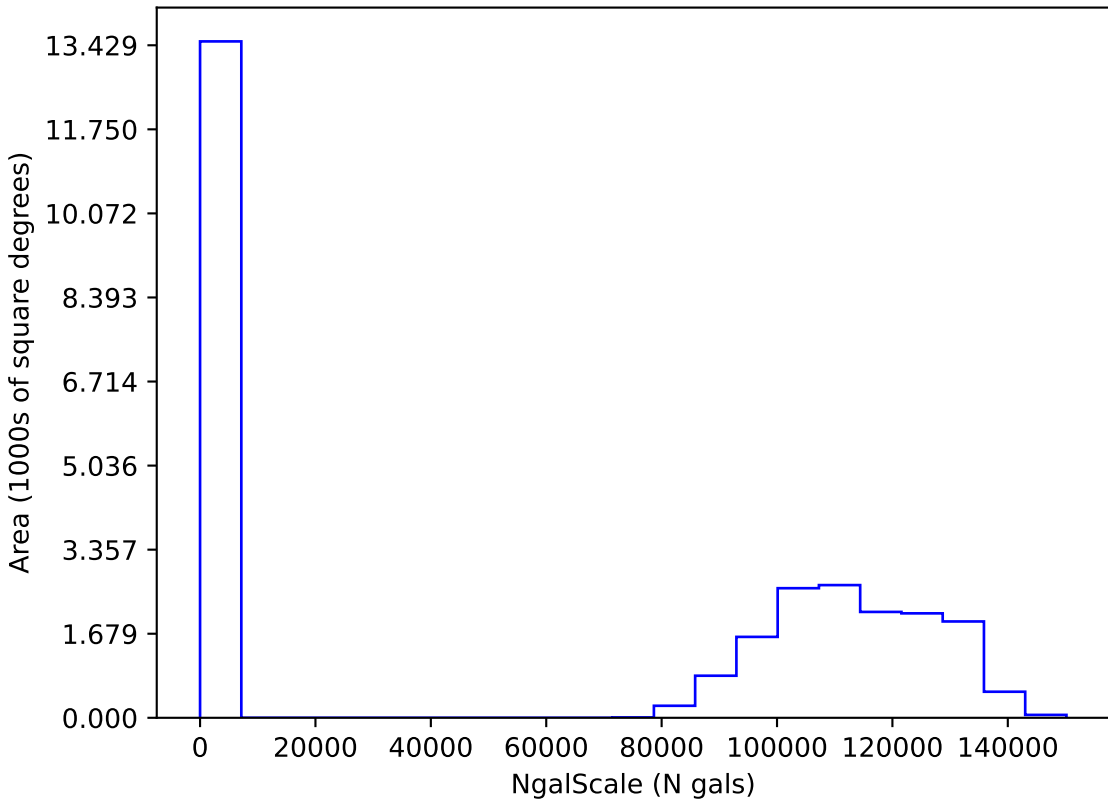
too_elab_heavy_r64_d2_griz_v3.4_10yrs i: NgalScale
