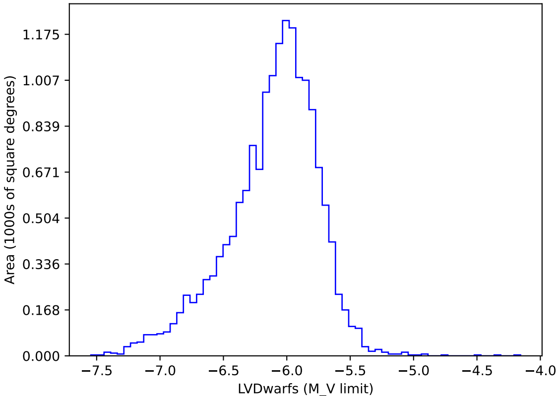
too_elab_heavy_r64_d2_griz_v3.4_10yrs gi: LVDwarfs
