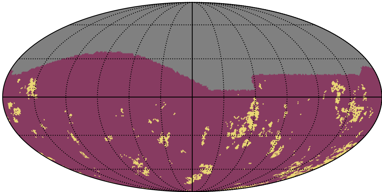
too_elab_heavy_r64_d2_griz_v3.4_10yrs g band: Gaps_7hr
