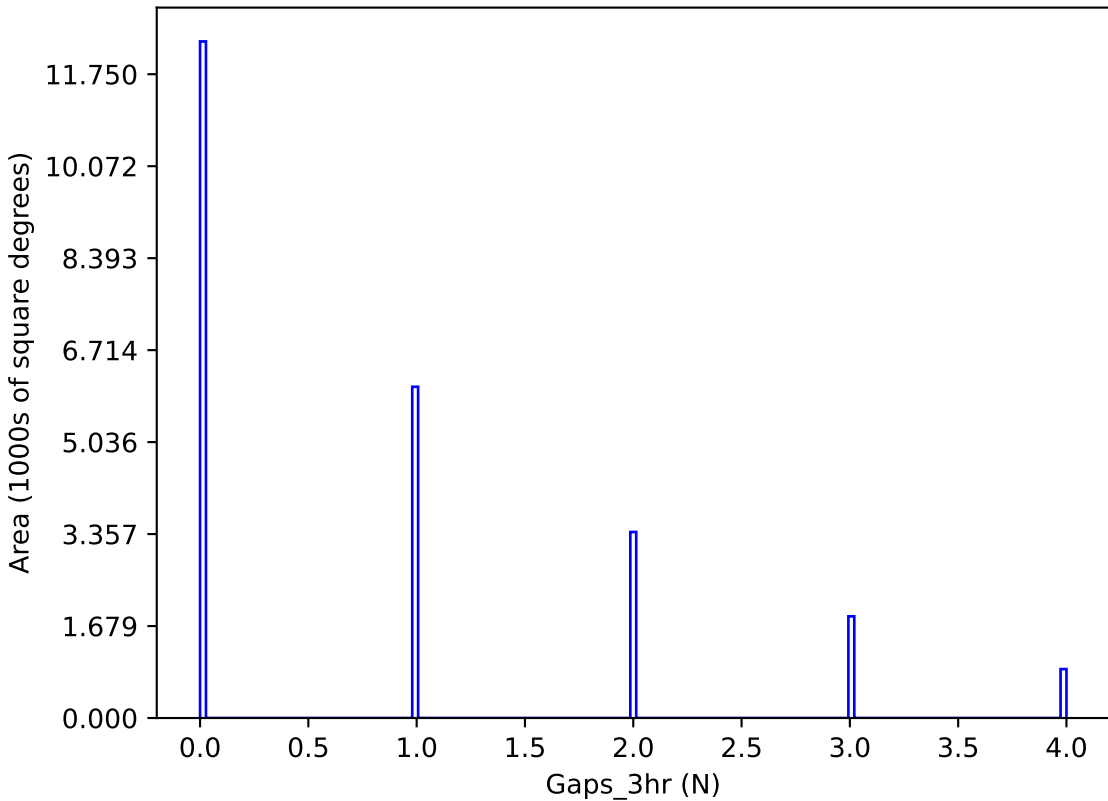
too_elab_heavy_r64_d2_griz_v3.4_10yrs y band: Gaps_3hr
