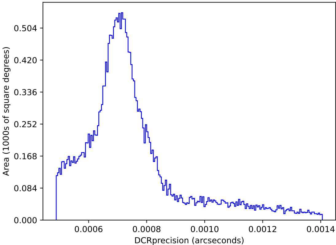
too_elab_heavy_r64_d2_griz_v3.4_10yrs : DCRprecision
