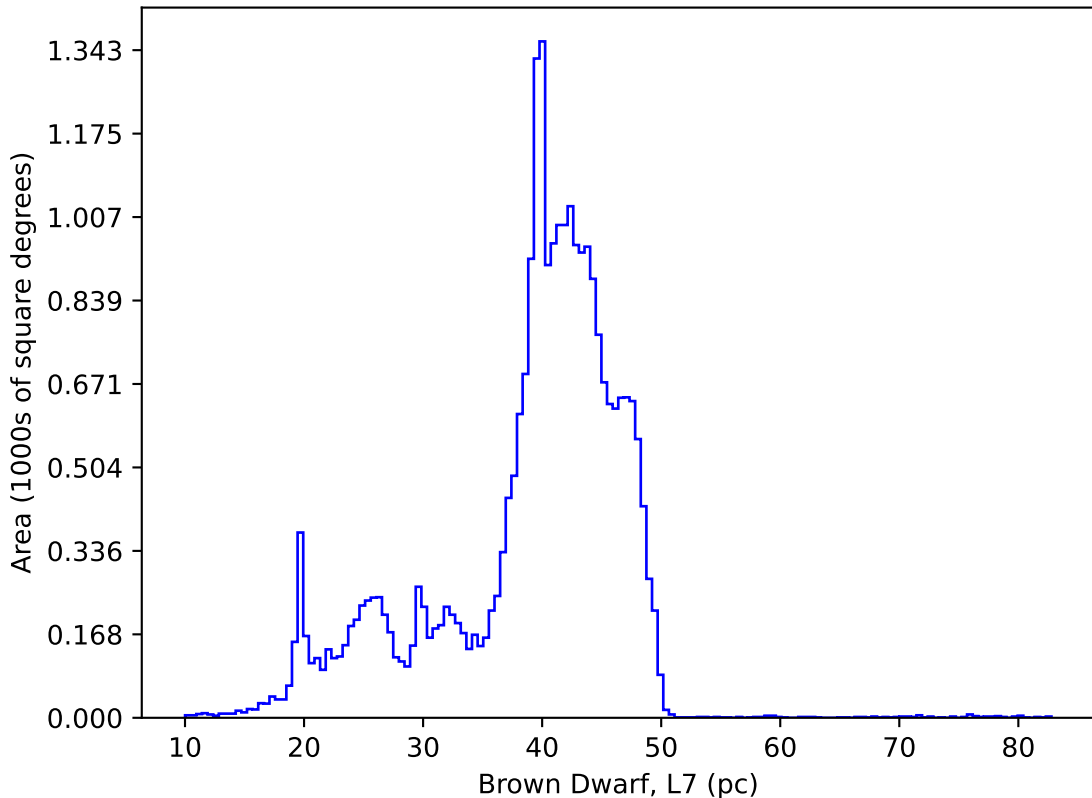
too_elab_heavy_r64_d2_griz_v3.4_10yrs : Brown Dwarf, L7
