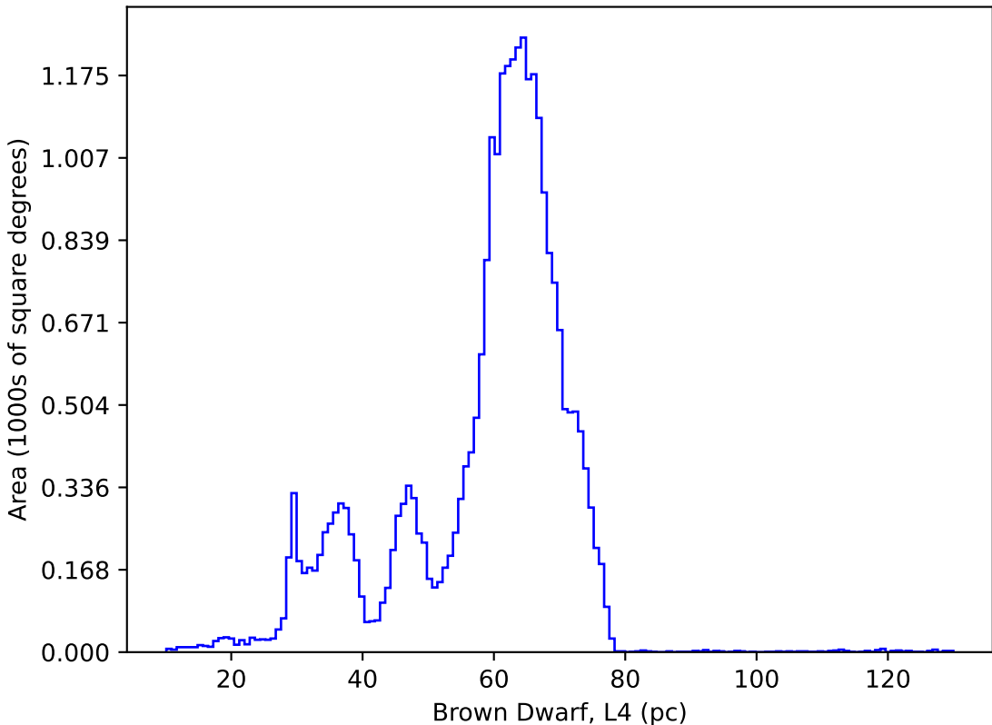
too_elab_heavy_r64_d2_griz_v3.4_10yrs : Brown Dwarf, L4
