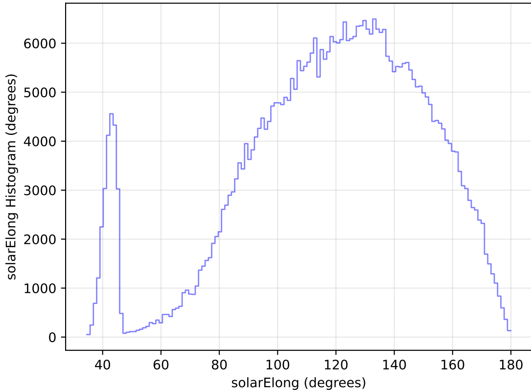
too_elab_heavy_r64_d2_griz_v3.4_10yrs WFD z band: solarElong Histogram
