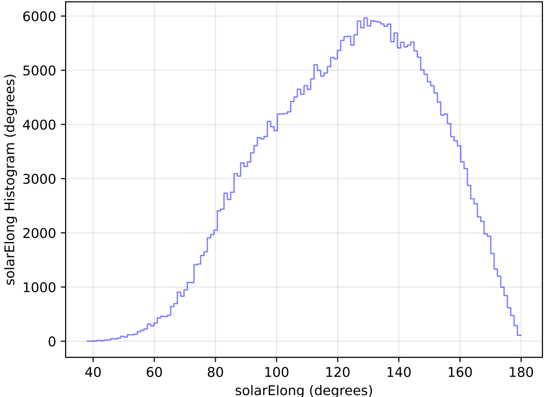
too_elab_heavy_r64_d2_griz_v3.4_10yrs WFD y band: solarElong Histogram
