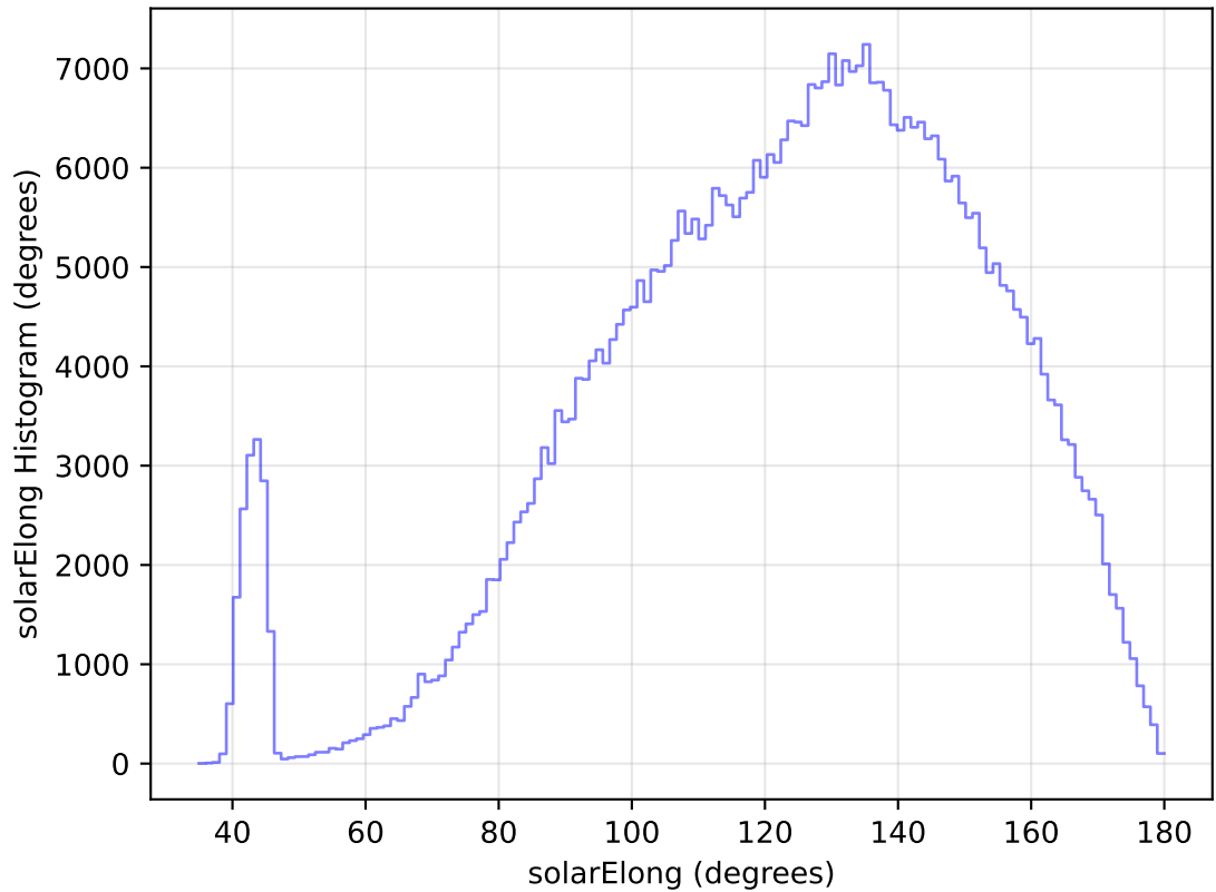
too_elab_heavy_r64_d2_griz_v3.4_10yrs WFD r band: solarElong Histogram
