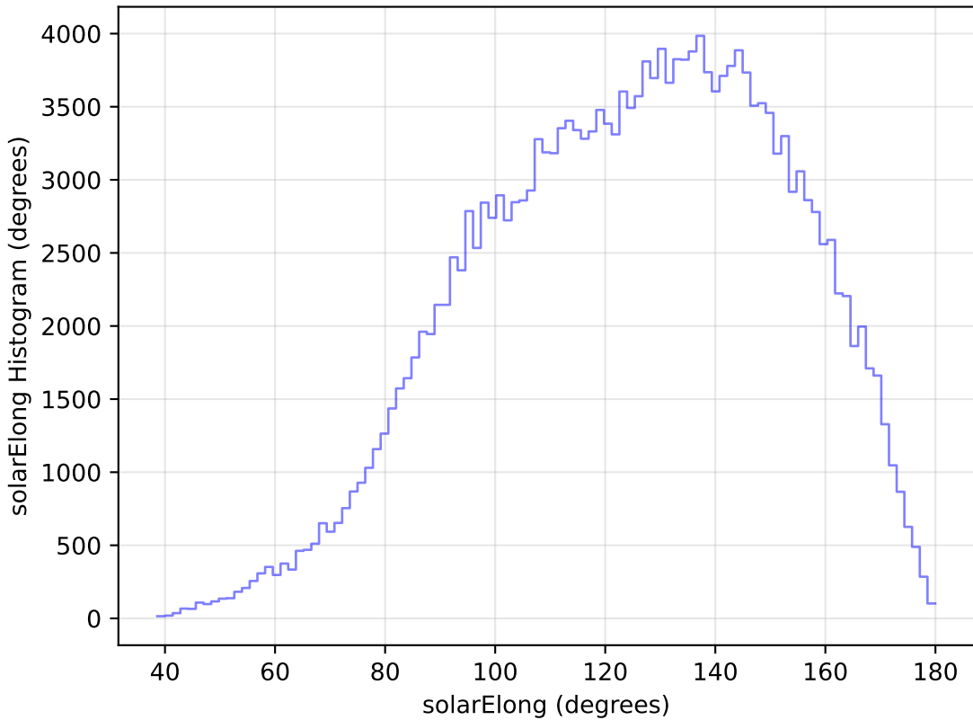
too_elab_heavy_r64_d2_griz_v3.4_10yrs WFD g band: solarElong Histogram
