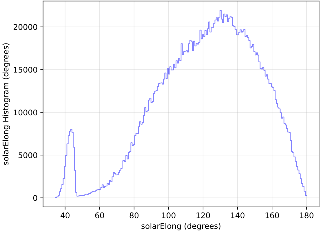
too_elab_heavy_r64_d2_griz_v3.4_10yrs WFD all bands: solarElong Histogram
