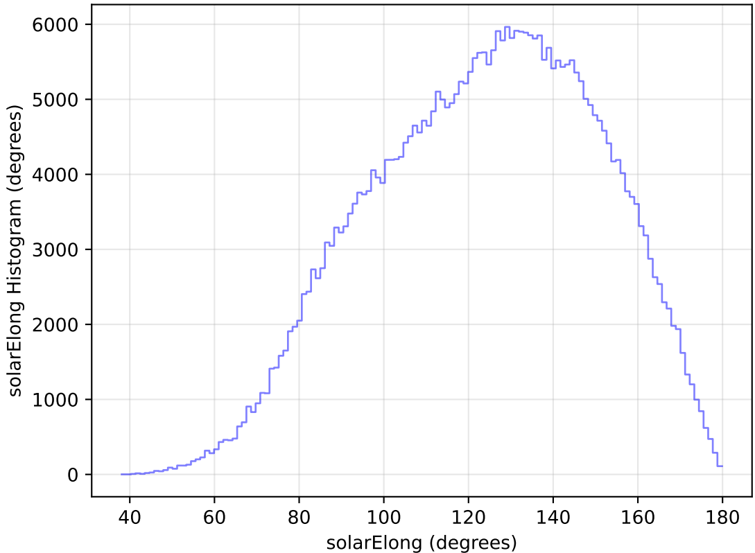
too_elab_heavy_r64_d2_griz_v3.4_10yrs All sky y band: solarElong Histogram
