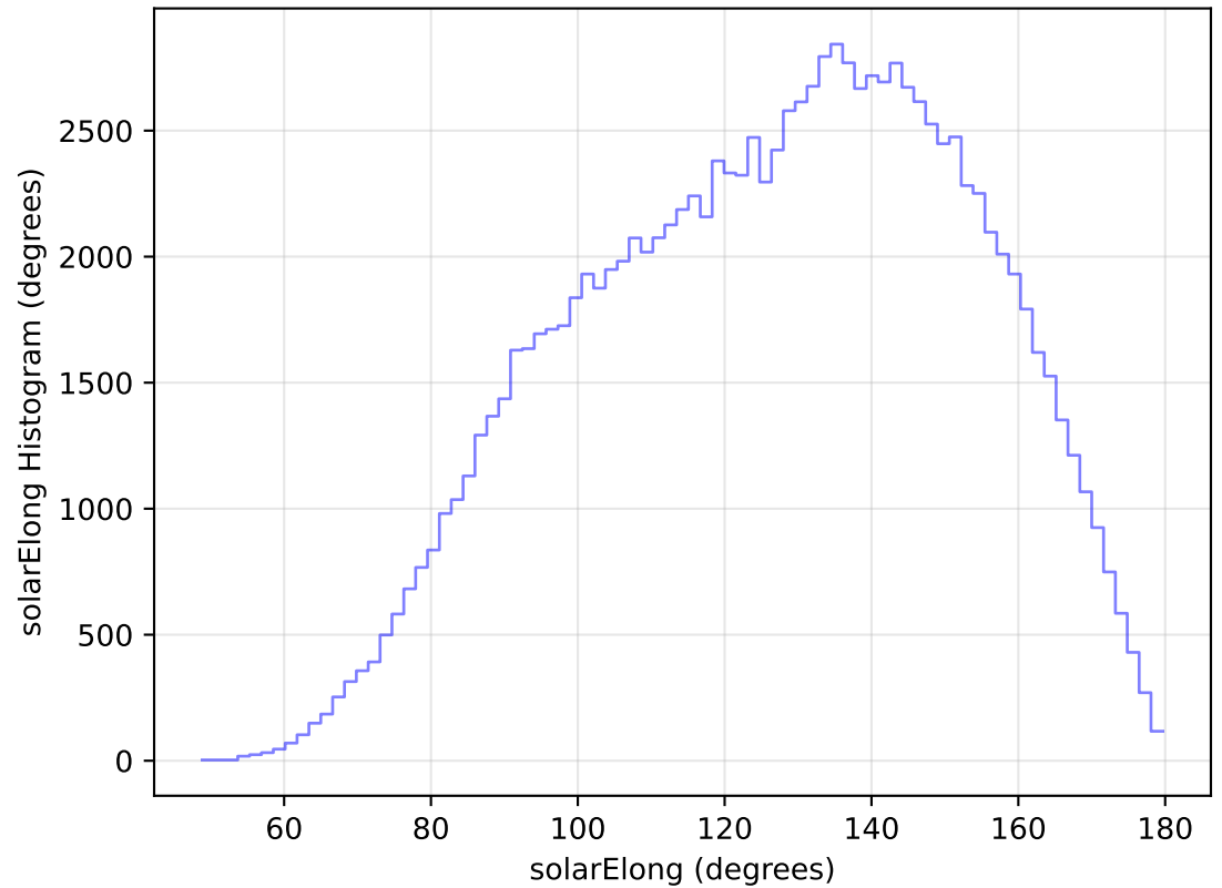
too_elab_heavy_r64_d2_griz_v3.4_10yrs All sky u band: solarElong Histogram
