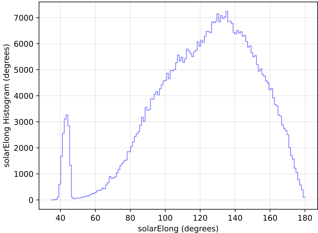
too_elab_heavy_r64_d2_griz_v3.4_10yrs All sky r band: solarElong Histogram
