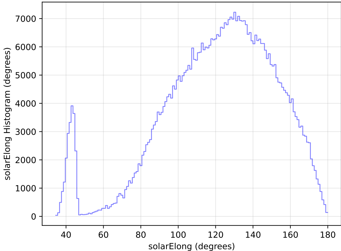
too_elab_heavy_r64_d2_griz_v3.4_10yrs All sky i band: solarElong Histogram
