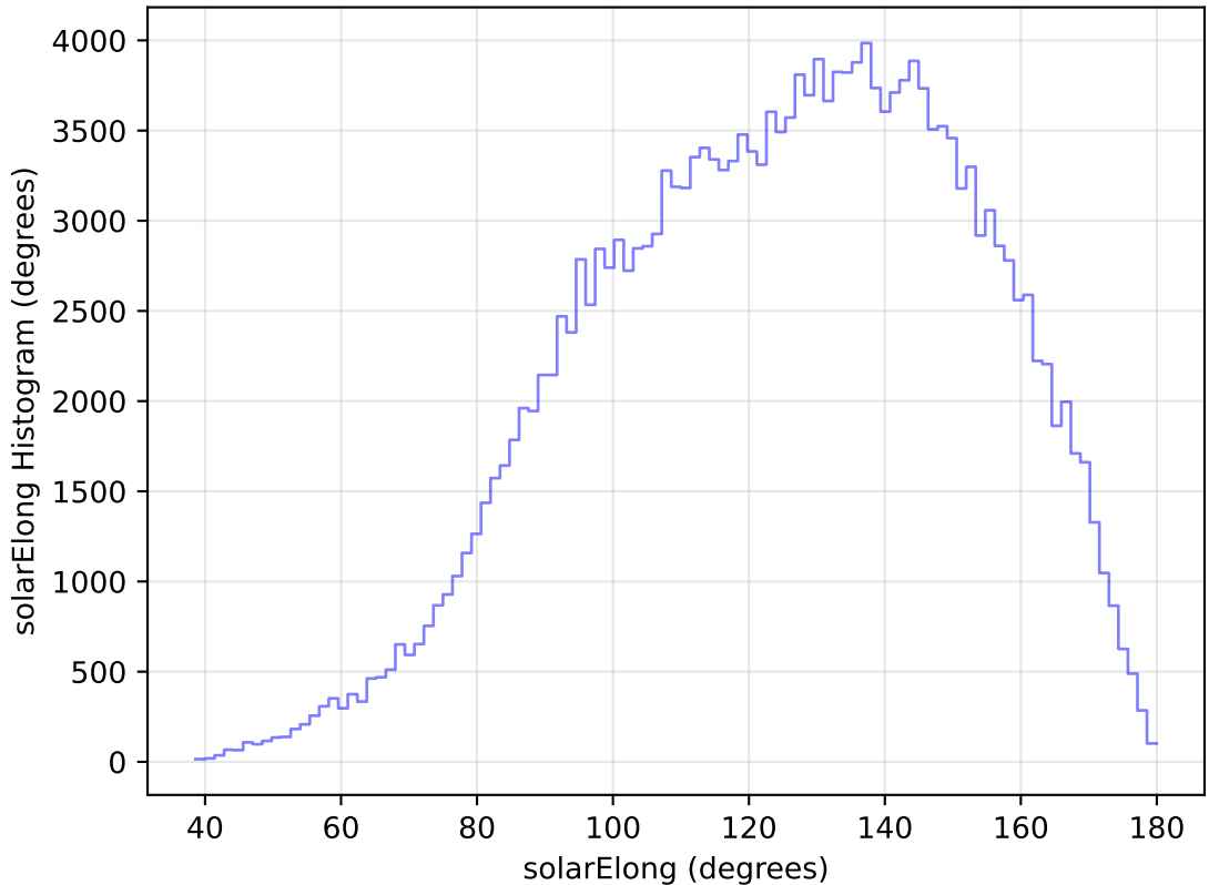
too_elab_heavy_r64_d2_griz_v3.4_10yrs All sky g band: solarElong Histogram
