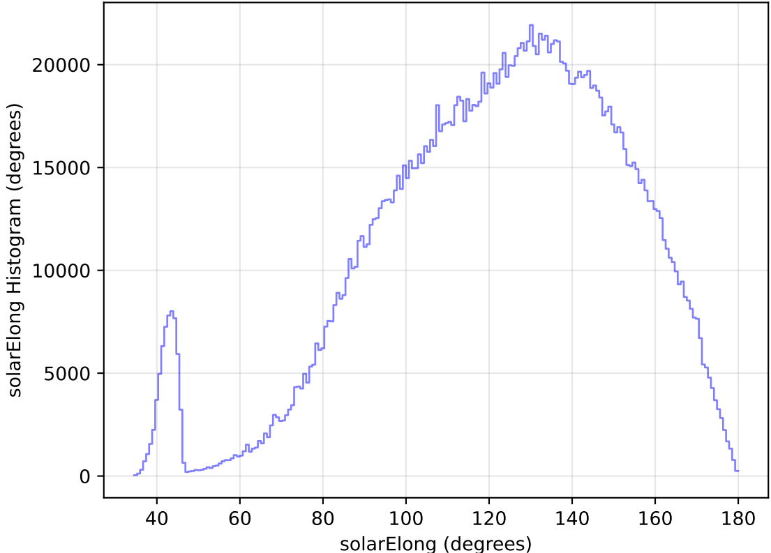
too_elab_heavy_r64_d2_griz_v3.4_10yrs All sky all bands: solarElong Histogram
