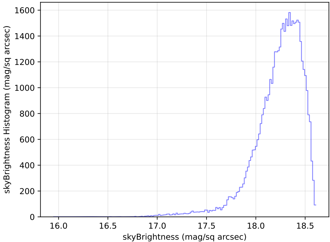
too_elab_heavy_r64_d2_griz_v3.4_10yrs Yr 1 y band: skyBrightness Histogram
