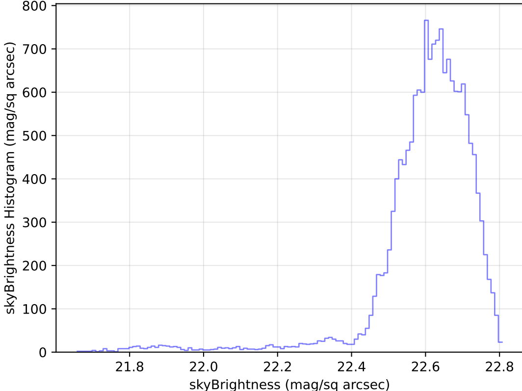
too_elab_heavy_r64_d2_griz_v3.4_10yrs Yr 1 u band: skyBrightness Histogram
