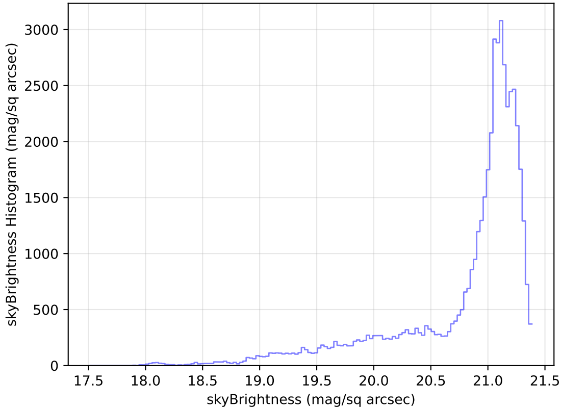
too_elab_heavy_r64_d2_griz_v3.4_10yrs Yr 1 r band: skyBrightness Histogram
